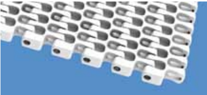
S18 | 44% open | Grid Top
